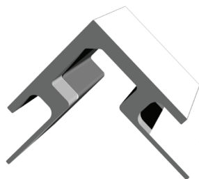
3-1/2" Outside Corner with Fin & J-Channel
