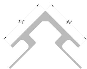
3-1/2" Outside Corner with Fin & J-Channel
